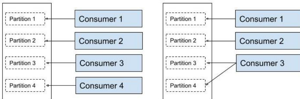
Optimal and non-optimal partitions assigning example
